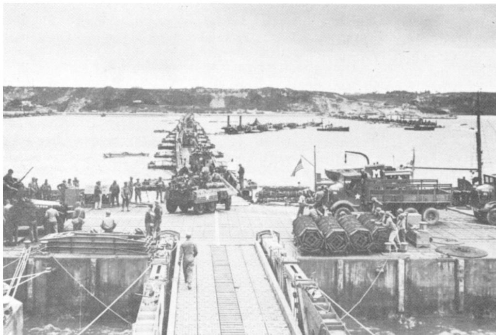
COMPLETED PIER OF THE MULBERRY in operation. Loaded vehicles coming ashore, above, and leaving Lobnitz pierhead, below.
